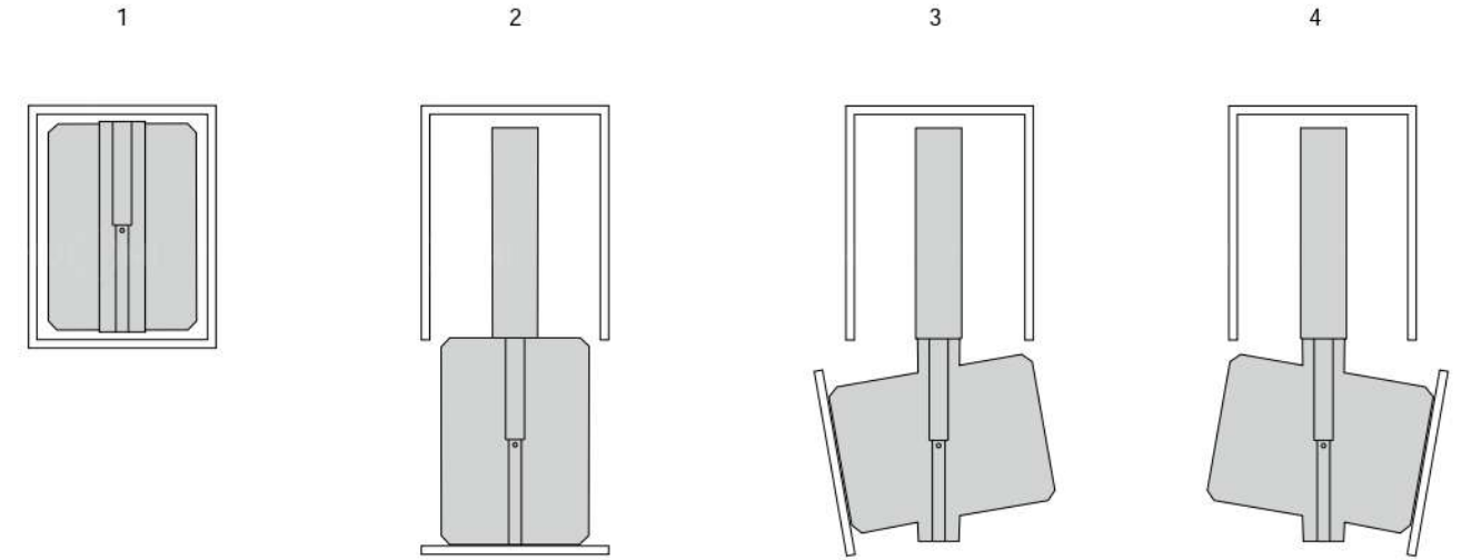
直拉式支架实现状态 / Straight Pull-out Tall Unit : 1, 2
